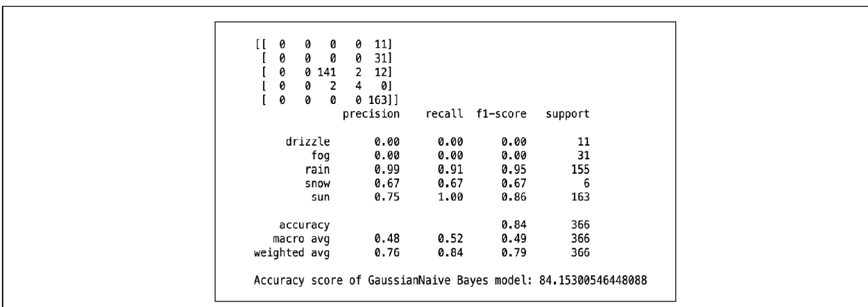
Figure 8: Accuracy score of Gaussian Naive Bayes
