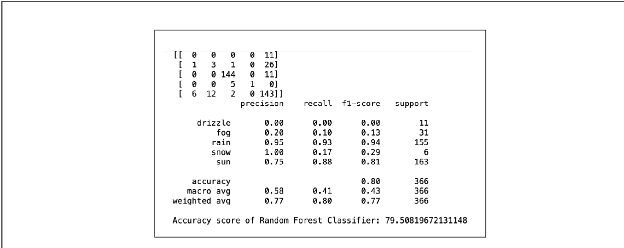
Figure 6: Accuracy Score of Random Forest Classifier
