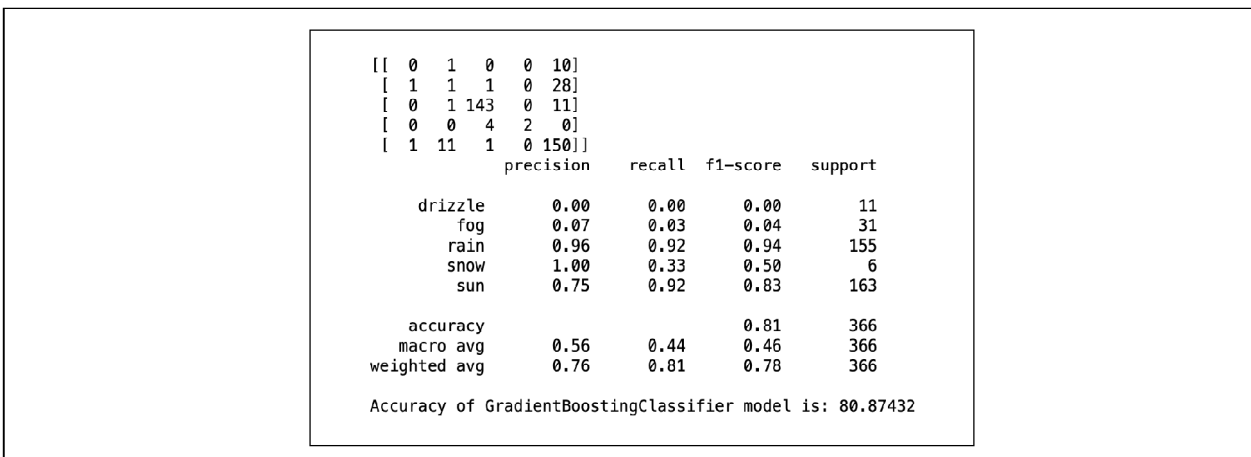
Figure 7: Accuracy Score of Gradient Boosting Classifier
