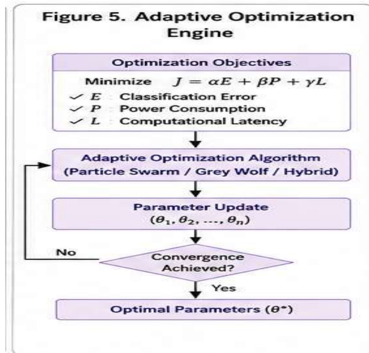
Figure 5. Adaptive Optimization Process for Parameter Tuning.
