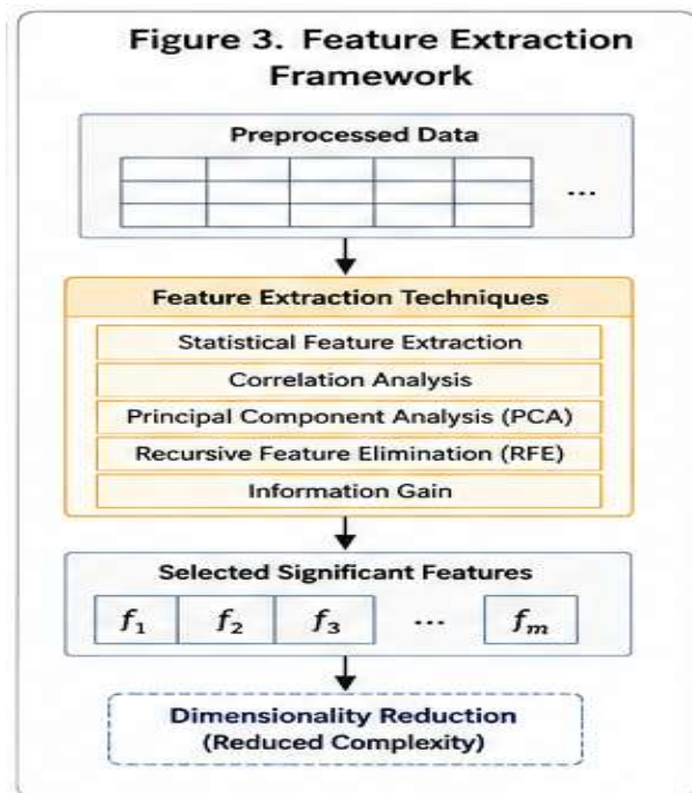
Figure 3. Significant Feature Extraction and Dimensionality Reduction Process.
