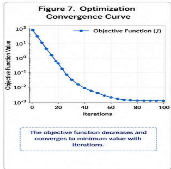
Figure 7. Convergence Characteristics of the Adaptive Optimization Algorithm.
