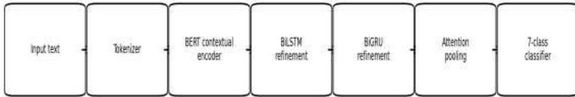
Figure 2. Proposed BERT-BiLSTM-BiGRU-attention architecture. This is a model schematic, not an empirical result.
