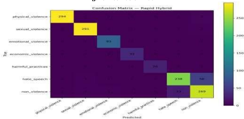
Figure 4. confusion matrix
