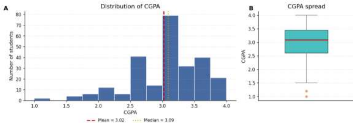
Figure 1. Distribution and Spread of Student Academic Performance: (A) Distribution of CGPA; (B) CGPA Spread.
