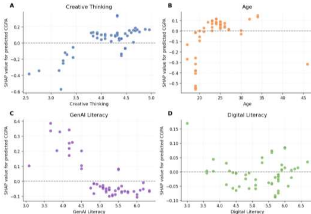
Figure 5. SHAP Dependence Patterns for Major Predictors of Academic Performance: (A) Creative Thinking; (B) Age; (C) GenAI Literacy; (D) Digital Literacy.
