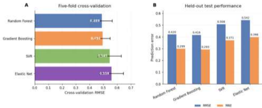
Figure 2. Predictive Performance of Machine-Learning Models: (A) Five-Fold Cross-Validation RMSE; (B) Held-Out Test RMSE and MAE.
