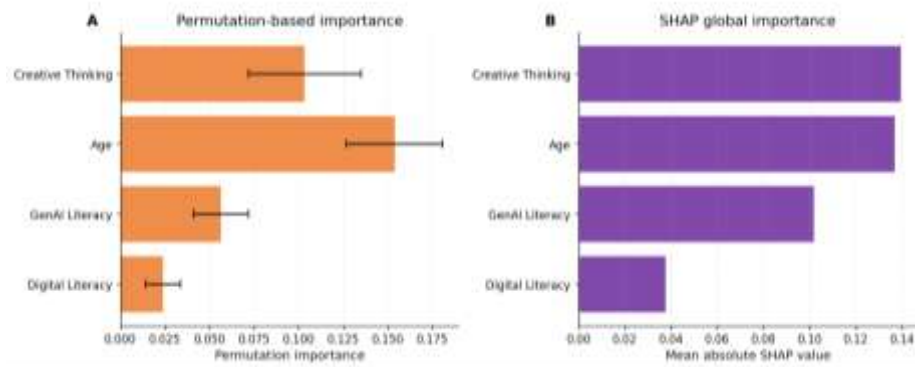
Figure 4. Global Importance of Academic Performance Predictors: (A) Permutation-Based Predictor Importance; (B) SHAP Global Predictor Importance.
