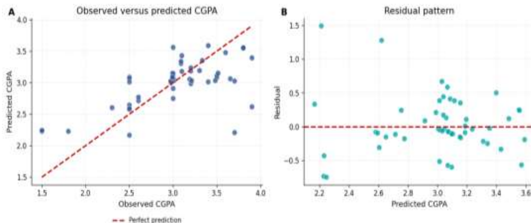
Figure 3. Random Forest Prediction and Residual Diagnostics: (A) Observed Versus Predicted CGPA; (B) Residual Pattern Across Predicted CGPA.
