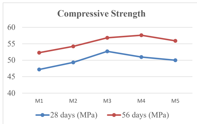
Fig.5: Compressive strength development at 28days vs 56 days
