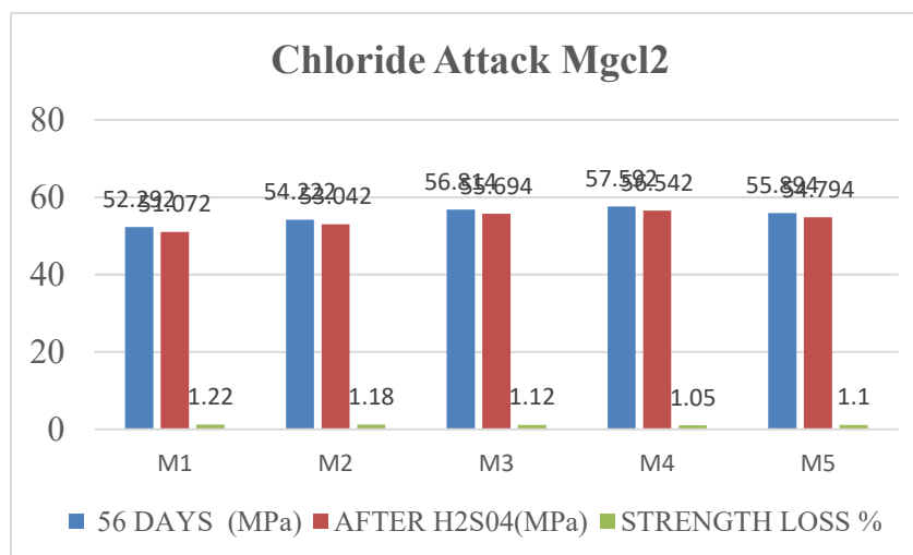
Fig.9: Chloride Attack Resistance
