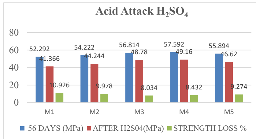
Fig.8: Acid Attack Resistance
