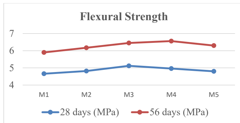
Fig.7: Flexural Strength Test at 28days vs 56 days
