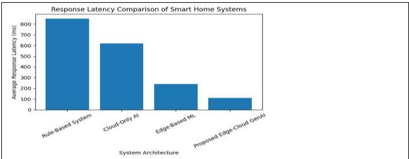
Fig. 2. Response Latency Comparisons of Smart Home Systems
